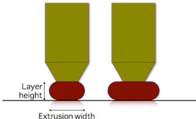
Figure 2.64: Extrusion Width.
